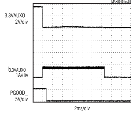
3.3VAUXO_CURRENT FOLDBACK
