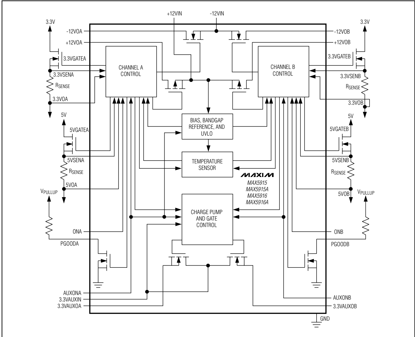
Functional Diagram
