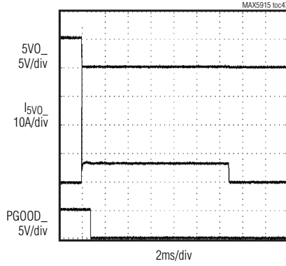
5VO_CURRENT LIMIT
