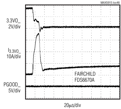
3.3VO_IMMEDIATE SHORT-CIRCUIT RESPONSE
