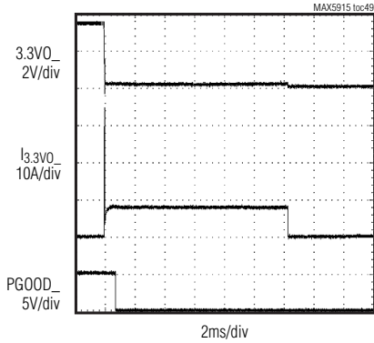
3.3VO_CURRENT LIMIT
